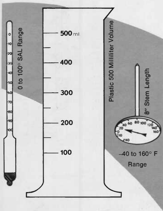
Figure 2. Equipment for measuring salt concentration in brine. Left, salometer; center, graduate cylinder; right, dial thermometer.
