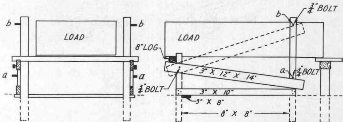
Figure 2.--Truck-loading scaffold using lever-arm support. Bolt a locks the lever arm in position to support the load, bolt b is a stop for the lever arm as the load is eased on to the truck.
