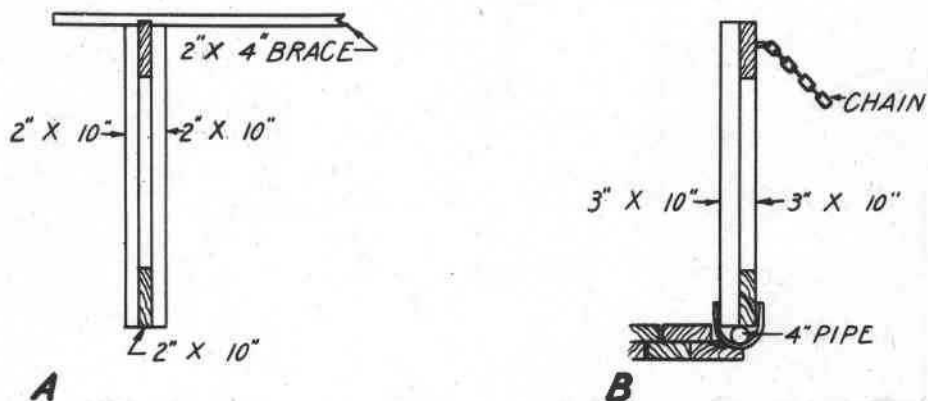
Figure 4.--Details of two types of gate frames. A, gate frame supported by notched 2-by-4; B, gate frame supported by chain and hinged on a pipe.
