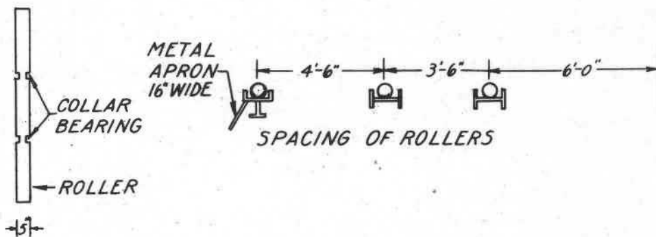
Figure 5.--Truck equipped with rollers for ease in loading and unloading, with details of truck roller and roller spacing.
