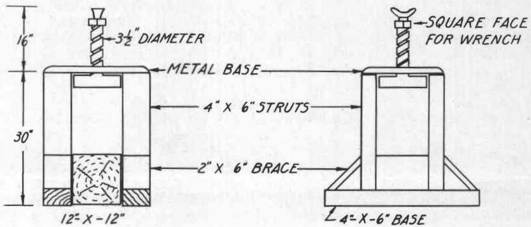
Figure 1.--Truck-loading scaffold using portable jacks and details of the standards in which the jacks are mounted.
