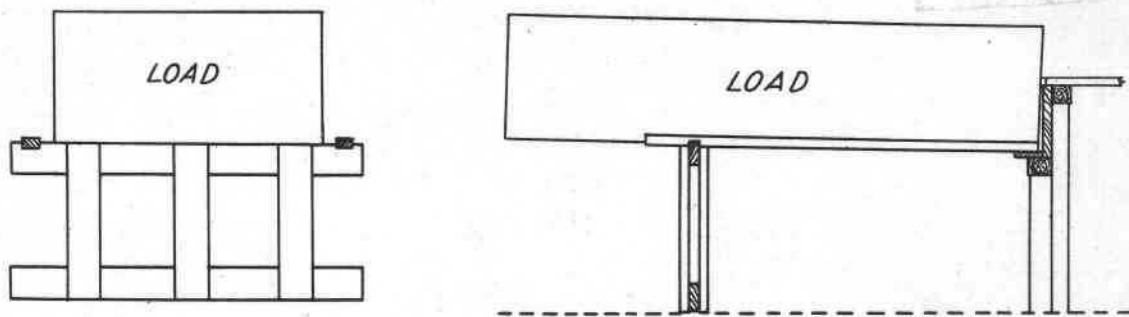
Figure 3.--Truck-loading scaffold using gate-frame support.
