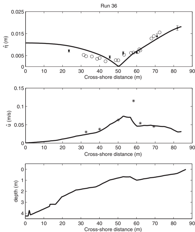
FIG. 1. (Top) cross-shore variation of \hat{\eta} , model (solid line) data (circles), error bars indicate variability for repeated measurements; (middle) cross-shore variation of \hat{u} , model (solid line) data (*); (bottom) fixed, barred beach bathymetry.
