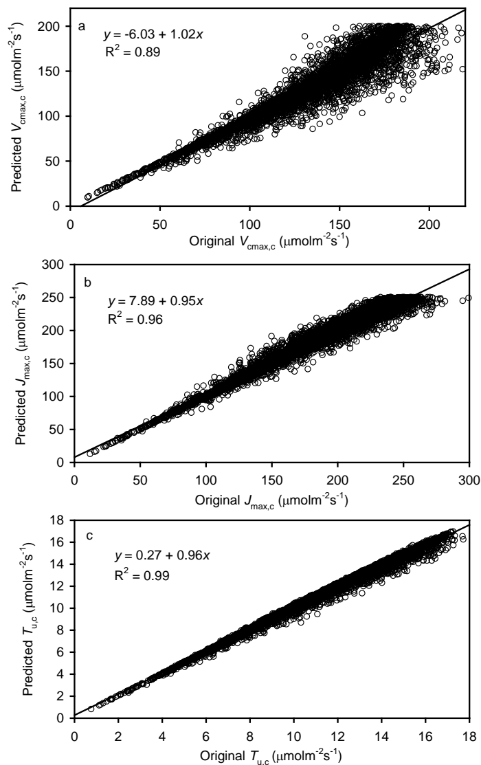
Figure S1. Comparison of predicted vs. original A/C_c -based V_{cmax} (a), J_{max} (b) and TPU (c) for the simulated A/C_i curve datasets. The prediction was calculated with the conversion function derived from the actual A/C_i curve measurements.
