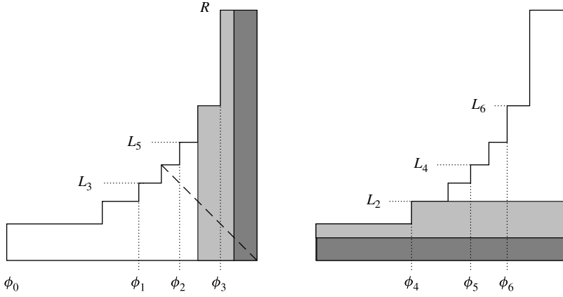
FIGURE 1. Natural extension for n = 5 . The region initially lying over \Delta_1 and its image are shown in white; the region over \Delta_2 and its image are shown in light gray; and the region above \Delta_k with k > 2 and its image are shown in dark gray. The anti-diagonal y = -x (dashed) is also shown.
