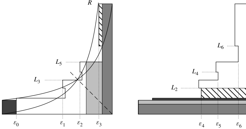
FIGURE 2. Natural extension of domain \Gamma , for accelerated map, n = 5 . The region initially lying over the accelerated subinterval is shaded darkest; the remainder lying above \Delta_1 is shown in white; the lower region over \Delta_2 is shown in light gray; the high region over (part of) \Delta_2 is shown lined; and the region above \Delta_k with k > 2 is shown in medium gray. Likewise their images. Curves corresponding to \theta(x, y) = \tau , y = -x (dashed) and related to \theta(\mathcal{T}^{-1}(x, y)) = \tau are also shown.
