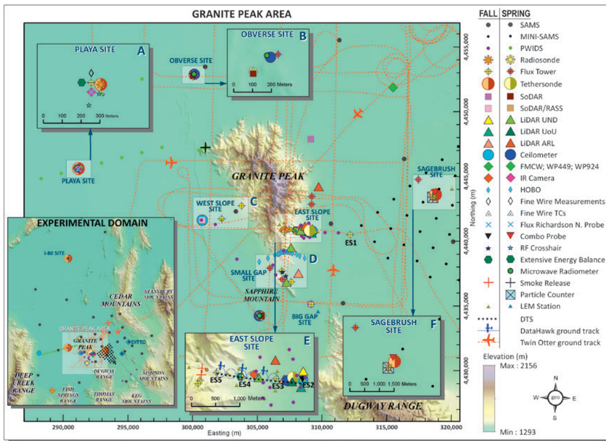
FIG. 3. Instrument placement during fall and spring campaigns. Insets provide details of IOSs as well as the full experimental domain (bottom-left inset). Only the additional instruments deployed (or relocated) for the spring experiment are shown under the “spring” column (courtesy of Dott. Ing. Roberto Perrone).
