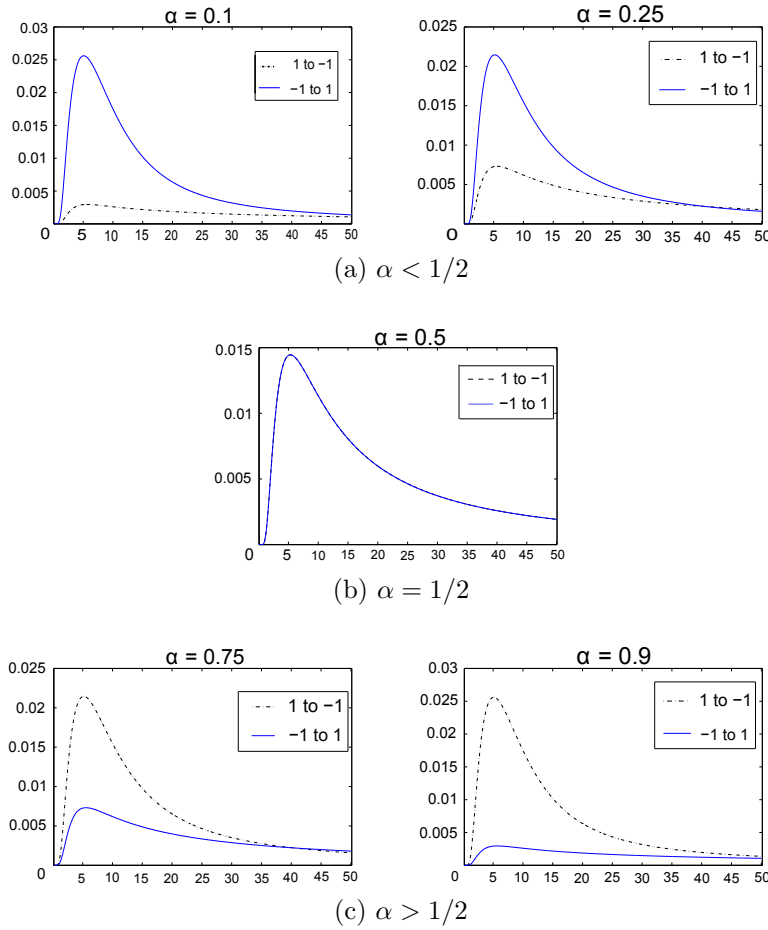
FIGURE 2: The densities P_{-1}(T_1^{(\alpha)} \in dt) (solid) and P_1(T_{-1}^{(\alpha)} \in dt) (dashed) for different values of \alpha .
