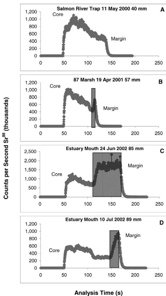
FIGURE 3.—Plots of strontium count rates versus analytical times (otolith radial distances) in four Salmon River Chinook salmon otoliths (A)–(D). The shaded boxes represent periods of estuary residence.
