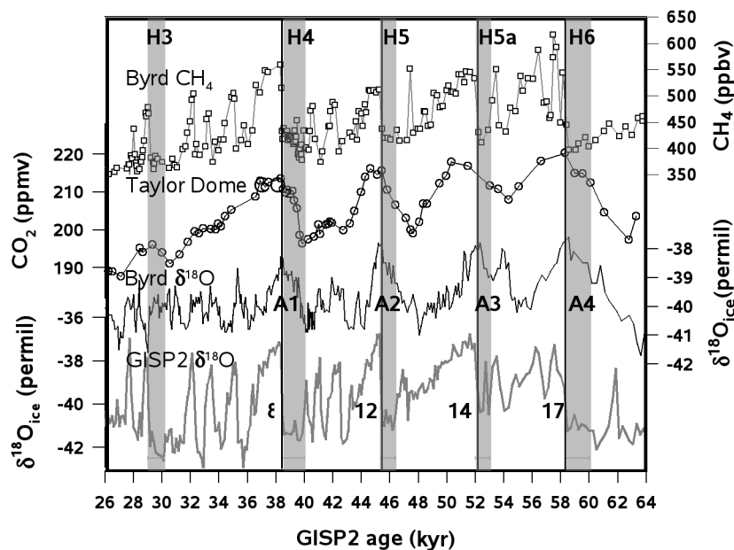
Figure 1. Comparison of atmospheric \text{CO}_2 and climate changes during the last ice age from Ahn and Brook (in press). Open square, \text{CH}_4 from Byrd ice core, Antarctica [ Blunier and Brook , 2001]; open circle, \text{CO}_2 from Taylor Dome, Antarctica [ Indermühle et al. , 2000]; black line, \delta^{18}\text{O}_{\text{ice}} , as a proxy of surface temperature, from Byrd station, Antarctica [ Johnsen et al. , 1972] on the timescale of Blunier and Brook [2001]; gray line, \delta^{18}\text{O}_{\text{ice}} from Greenland Ice Sheet Project 2 (GISP2) ice core (Summit, Greenland) [ Grotes et al. , 1993]. \text{CO}_2 from Taylor Dome is synchronized with GISP2 age ( Ahn and Brook , in press) using \text{CH}_4 from Taylor Dome [ Brook et al. , 2000] and \text{CO}_2 from Byrd station [ Ahn and Brook , in press; Nefstel et al. , 1988]. Vertical lines denote the peak of Antarctic warm events A1-A4 which are associated with rapid transitions from a cold stadial to warm interstadial state in Greenland. Gray shaded bars represent Heinrich events [ Sarnthein et al. , 2001; Rashid et al. , 2003]. Dansgaard/Oeschger warm events 8, 12, 14 and 17 and Heinrich events 3, 4, 5, 5a and 6 are denoted by numbers. Note that following these stadial to interstadial transitions atmospheric \text{CO}_2 decreases gradually on a multi-millennial time scale.
