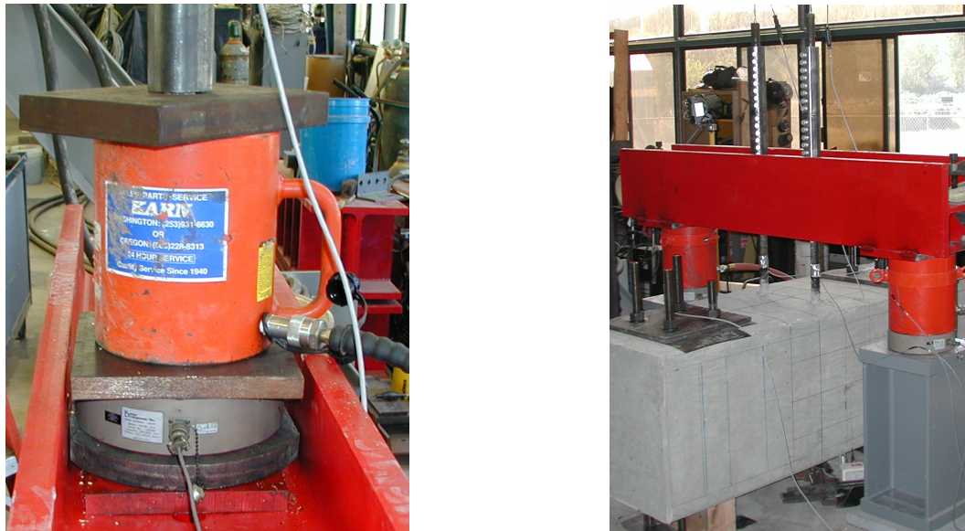
Fig. R9 - Typical Testing Setups for Series 1 and 2.
