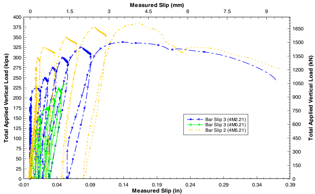
Fig. R18 - Maximum capacity comparison for inner bars of medium confinement specimens
