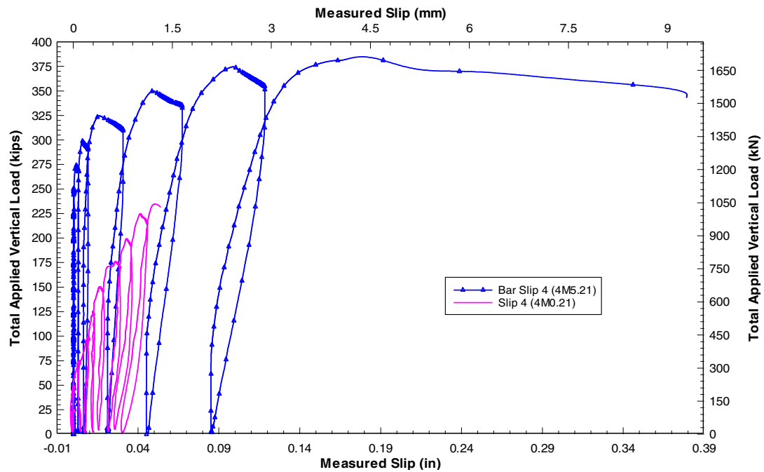
Fig. R17 - Maximum capacity comparison for outer bars of medium confinement specimens.
