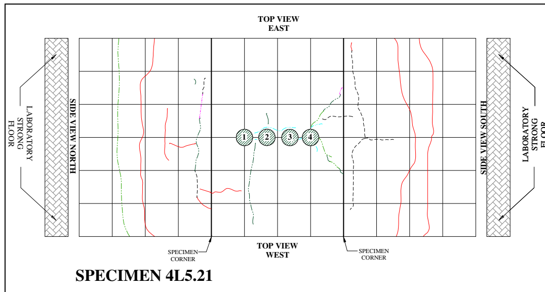
Fig. R24 - Specimen 4L5.21 crack map.
