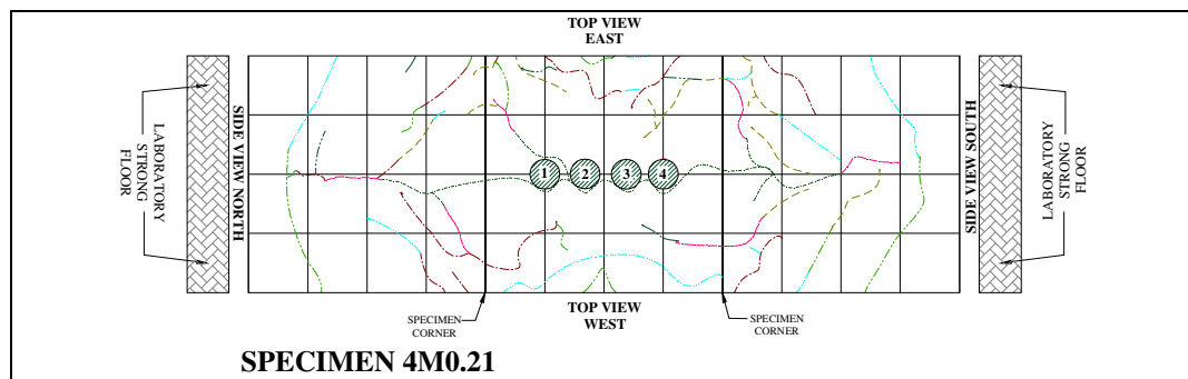
Fig. R25- Specimen 4M0.21 crack map.
