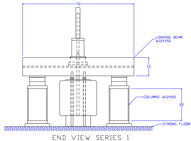
Fig. R11 - Typical Testing set up for Series 1 specimens.
