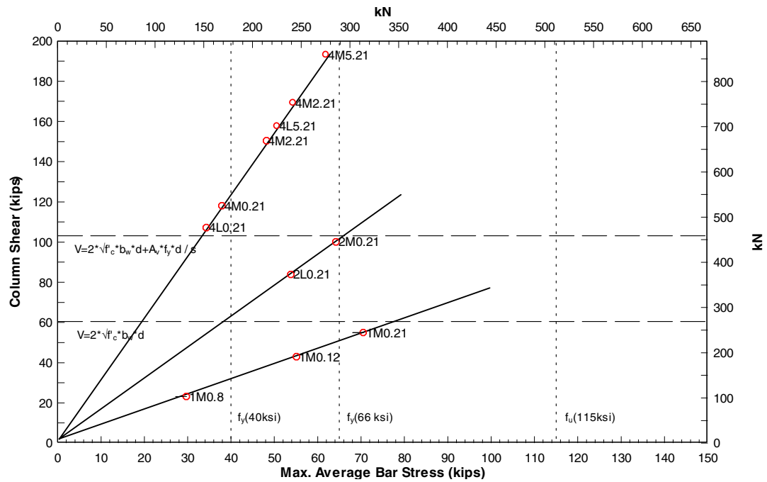
Fig. R37 - Maximum average bar stress in comparison to column shear demand.
