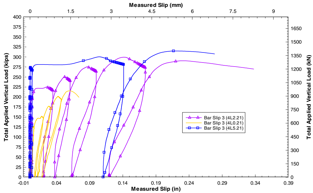
Fig. R16 - Maximum capacity comparison for inner bars of low confinement specimens.
