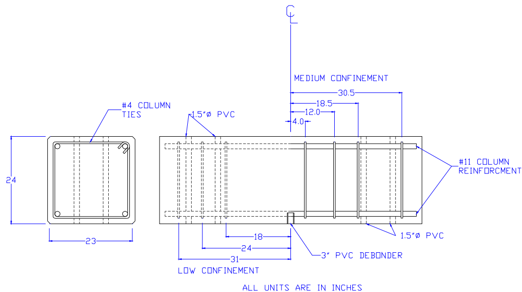
Fig. R3-Typical column reinforcing details for all specimens, both low and medium stirrups.
