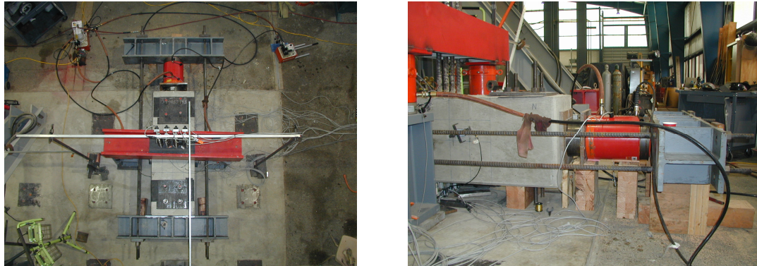
Fig. R10 - Typical plan and elevation views for Series 3.
