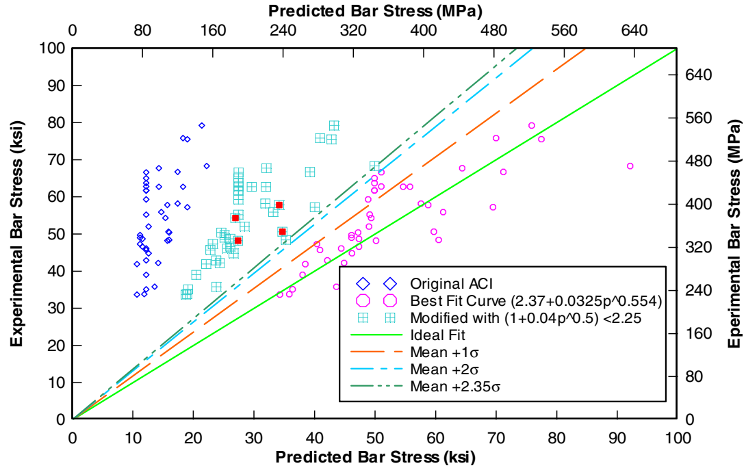
Fig. R41-Experimental and predicted bars stress plotted with standard deviation.
