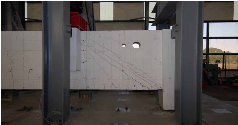
Fig.R2-Typical diagonal crack forming at column bent connection roller side reaction.
