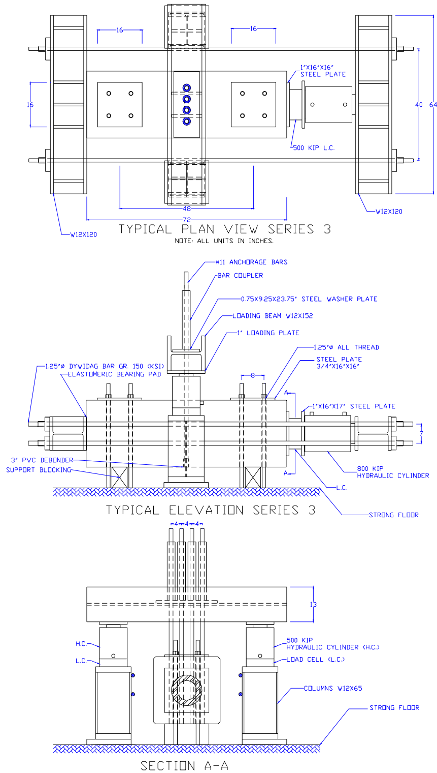
Fig. R13 - Typical testing setup for Series 3
