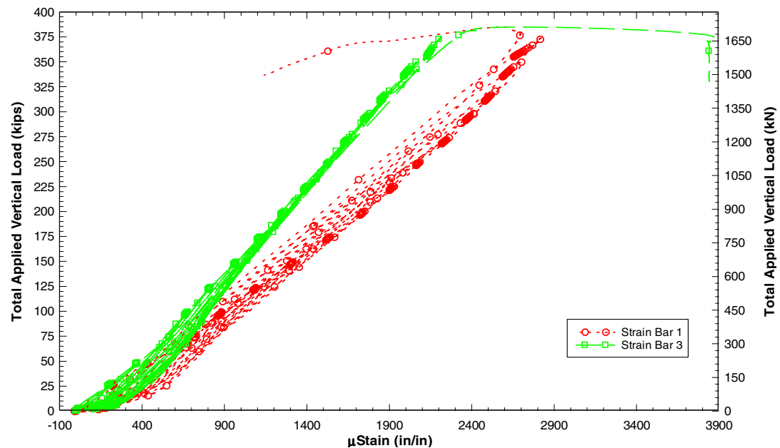
Fig. R34 - Strain for bars 1 and 3 of Specimen 4M5.21, Bar 1 pullout failure Bar 3 yielding.
