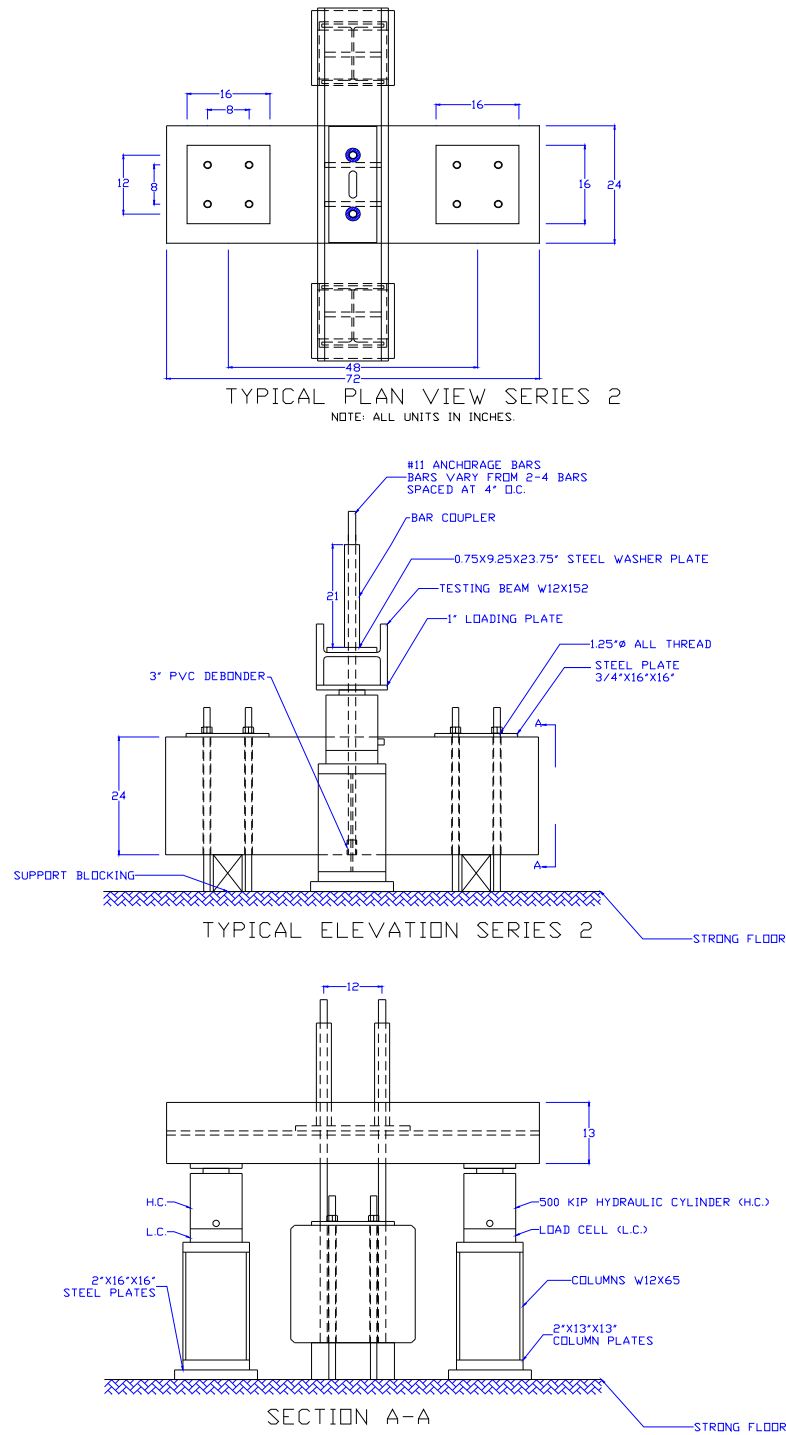
Fig. R12 - Typical testing setup for series 2 specimens (4 bar configurations not shown).
