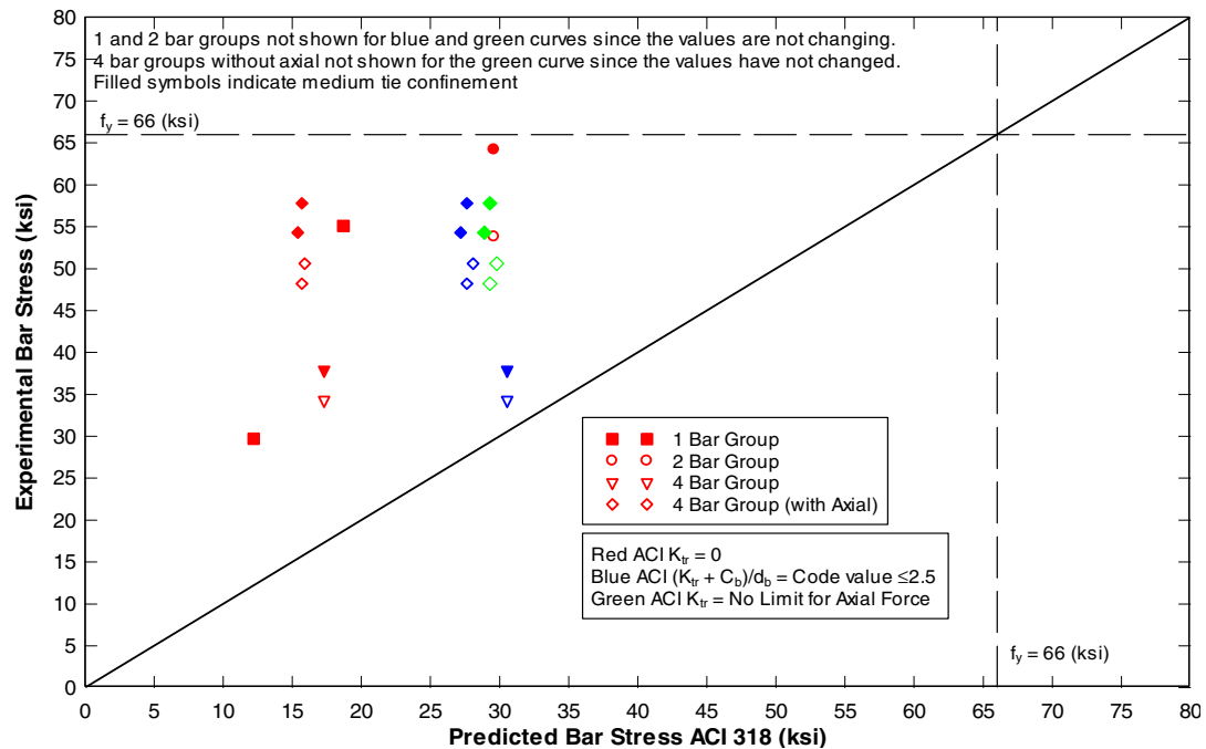
Fig. R39-Experimental bar stress in comparison to ACI 318-05 predicted bar stress.
