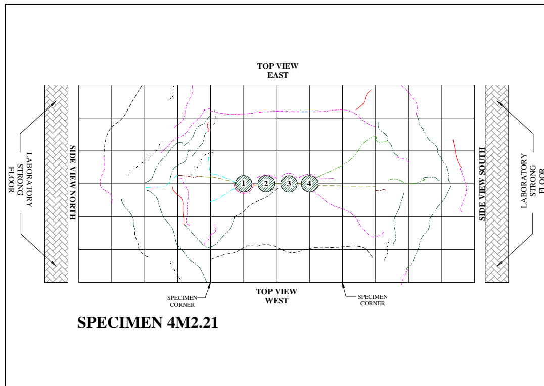
Fig. R26- Specimen 4M2.21 crack map.
