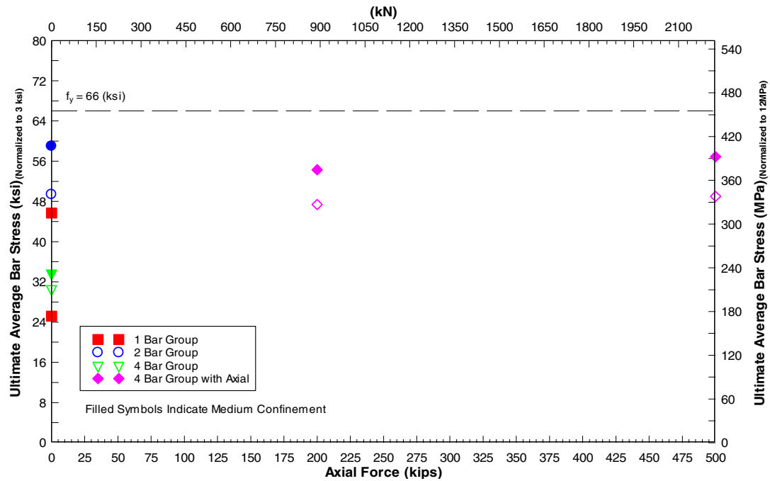
Fig. R36-Ultimate average bar stress normalized to Eq. 6 compared with axial force.
