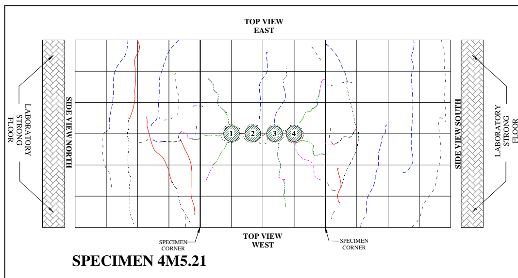
Fig. R27- Specimen 4M5.21 crack map.
