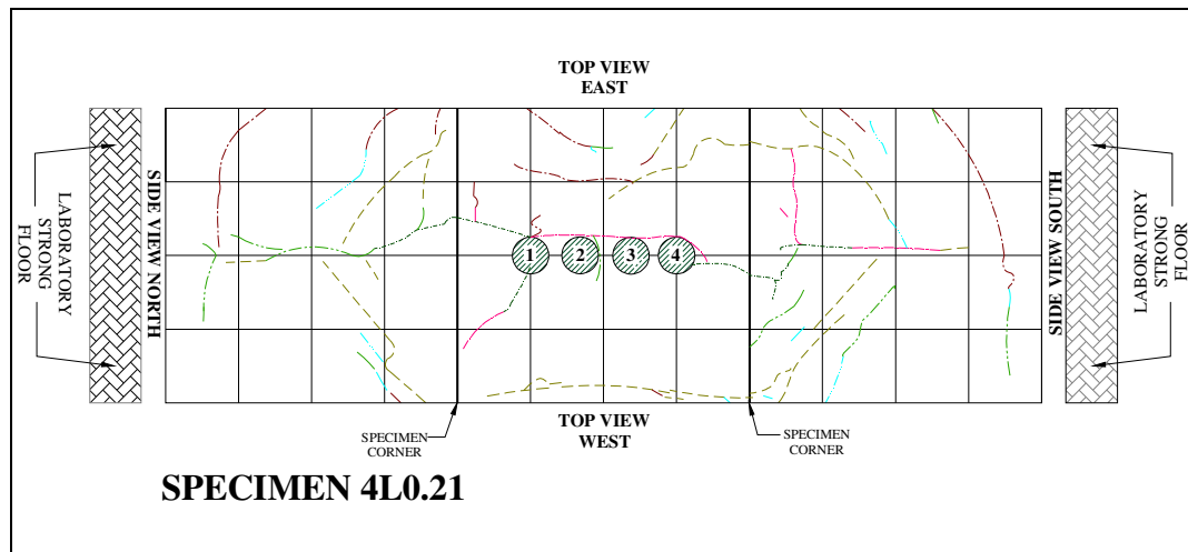
Fig. R22 - Specimen 4L0.21 crack map.
