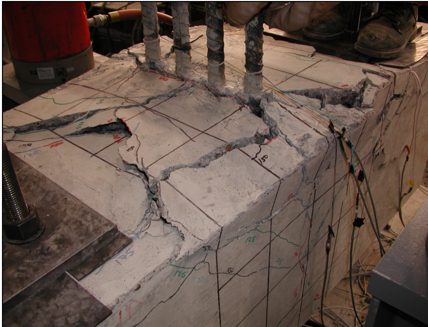
Fig. R31 - Typical pullout failure for series 2.
