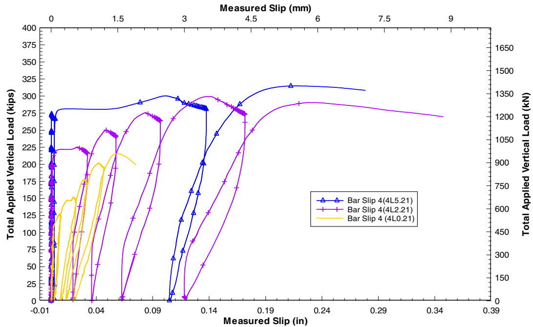
Fig. R15 - Maximum capacity comparison for outer bars of low confinement specimens.
