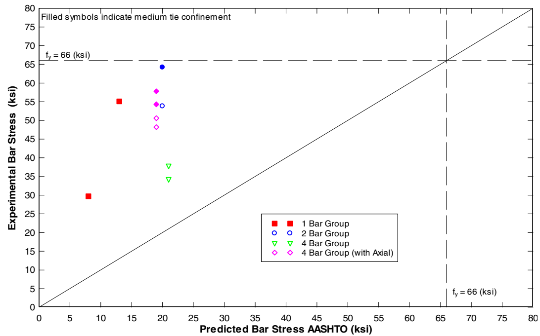
Fig. R38-Experimental bar stress in comparison to AASHTO predicted bar stress.
