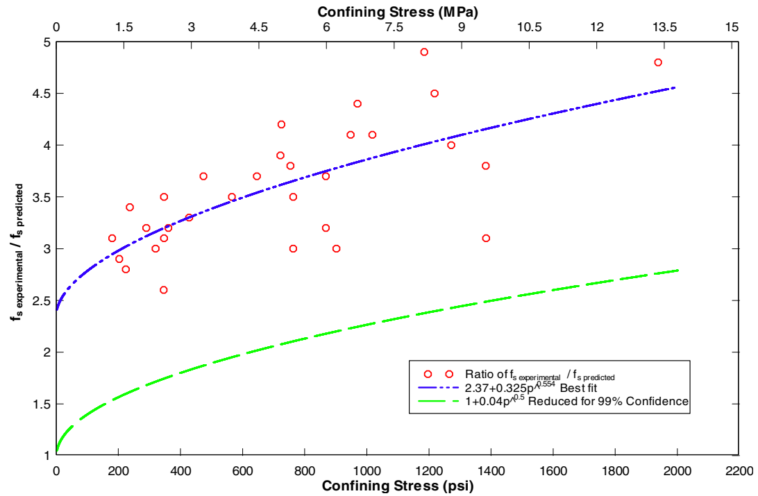
Fig. R40-Ratio of f_{s \text{ experimental}} / f_{s \text{ predicted}} versus confining stress, with best fit curve and with reduced curve.
