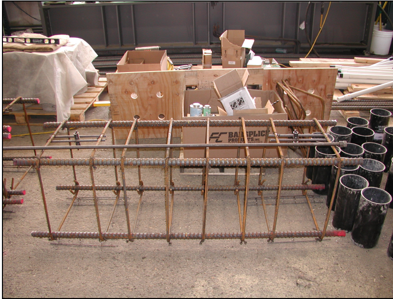
Fig. R5- Typical medium confinement column cage prior to casting.
