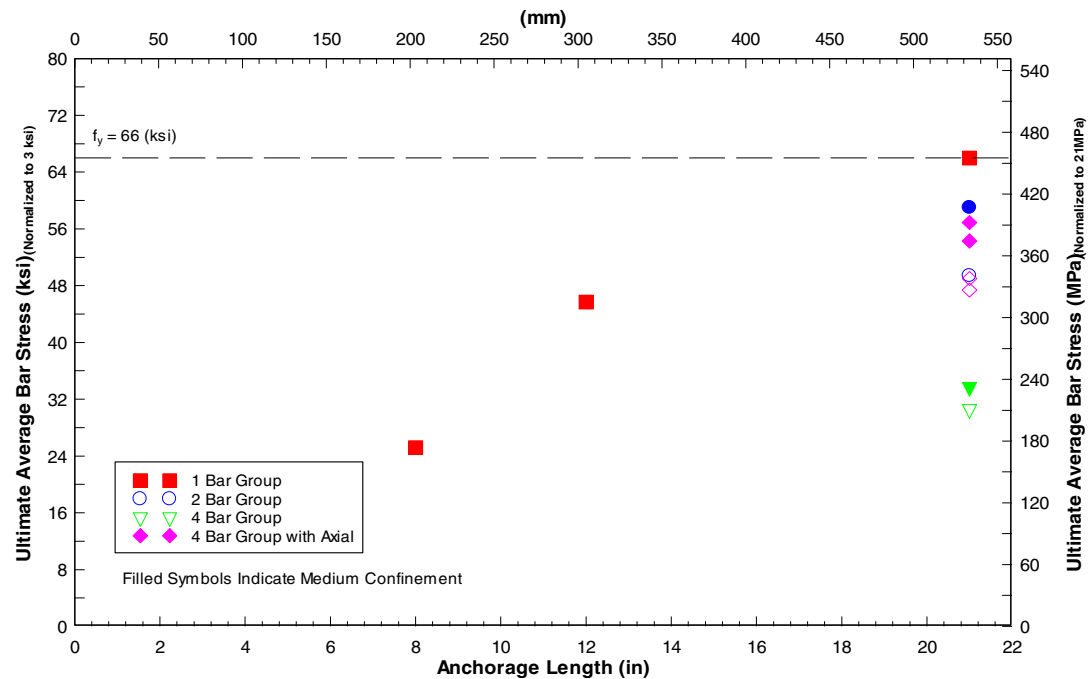
Fig. R35-Ultimate average bar stress normalized to Eq. 6 compared with anchorage length.
