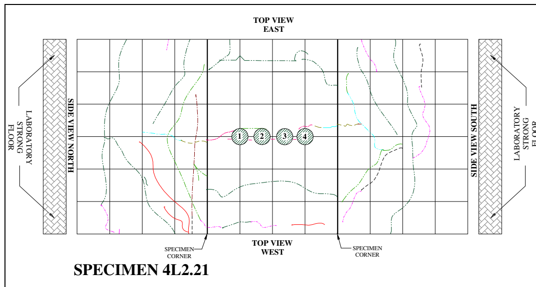
Fig. R23 - Specimen 4L2.21 crack map
