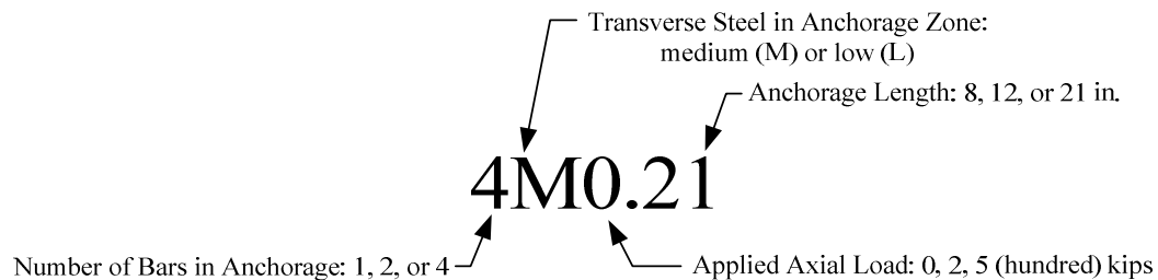
Fig. R4 - Specimen designation schematic.
