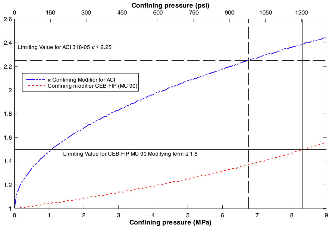
Fig. R42-Development length reduction factors proposed and CEB-FIP (MC 90).
