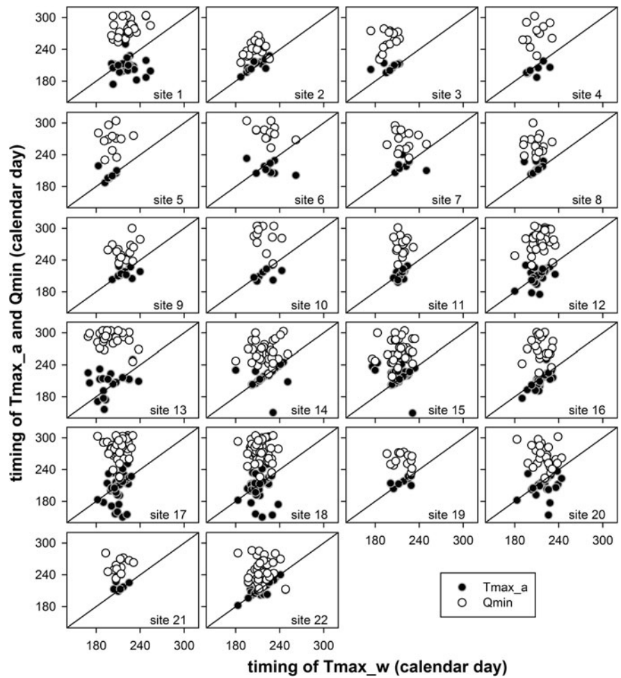
Fig. 2 Observed timing (calendar day) of the annual air temperature maxima ( T_{\max_a} ) and annual stream flow minima ( Q_{\min} ) compared to the timing of annual stream temperature maxima ( T_{\max_w} ). Each panel shows one site with one symbol for each year. Points located on the 1:1 line suggest complete synchrony. All symbols correspond to the 7-d MA event. A similar figure for the 1-d event is included in the Supplementary material
