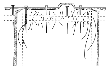
Figure 9. Pin to hold gathers before stitching.
