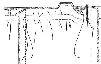
Figure 8. Fasten and pull bobbin threads to evenly distribute gathers.
