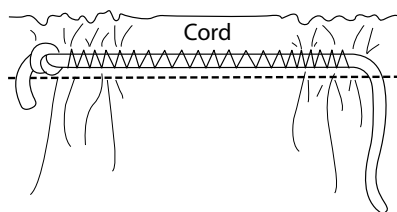
Figure 7. Zigzag stitching over a cord.
