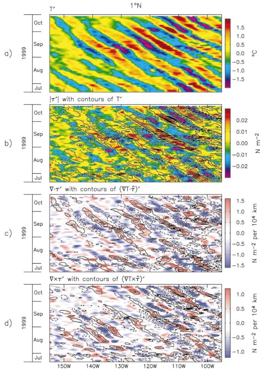
FIG. 14. Time-longitude plots along 1^{\circ}\text{N} on the north side of the cold tongue showing zonally high-pass filtered SST and wind stress fields: (a) perturbation SST; (b) perturbation wind stress magnitude with contours of perturbation SST overlaid; (c) perturbation wind stress divergence with contours of the perturbation downwind SST gradient, (\nabla T \cdot \hat{\tau})' , overlaid; and (d) perturbation wind stress curl with contours of the perturbation crosswind SST gradient, (\nabla T \times \hat{\tau})' \cdot \hat{k} , overlaid. Contour intervals are 0.5^{\circ}\text{C} in (b) and 0.4^{\circ}\text{C} (100 \text{ km})^{-1} in (c) and (d). For clarity, zero contours have been omitted from (b) to (d).
