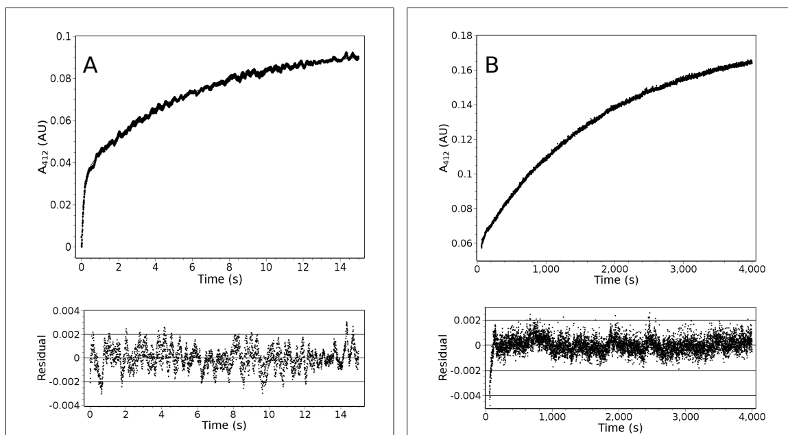
Figure 11. Alkylation of the wild-type hRXR \alpha LBD by DTNB under native conditions. 5.6 \mu M hRXR \alpha LBD and 1.11 mM DTNB. (A) Fast region fitted to eq. 2: D_1 = 0.0371 \pm 0.0004 AU, D_2 = 5.96 \pm 0.08 E-2 AU, k'_{obs} = 7.17 \pm 0.12 s ^{-1} , k''_{obs} = 0.173 \pm 0.001 s ^{-1} . (B) Slow region fitted to eq. 1: B = 0.11900 \pm 0.00004 AU, k_{obs} = 0.000562 \pm 0.000001 s ^{-1} .
