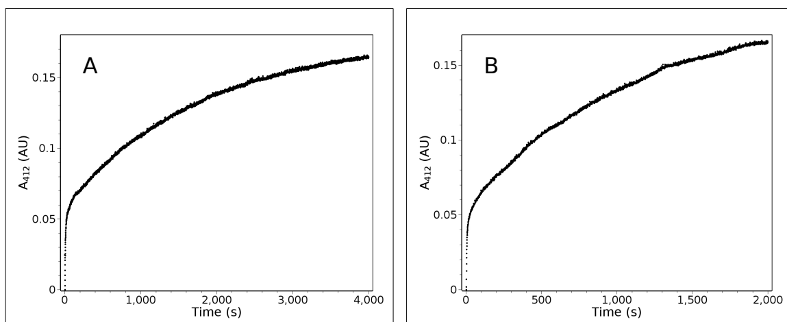
Figure 10. Alkylation of the wild-type hXR \alpha LBD by DTNB under native conditions. (A) 5.6 \mu\text{M} hXR \alpha LBD and 1.11 mM DTNB. (B) 5.6 \mu\text{M} hXR \alpha LBD and 2.78 mM DTNB.
