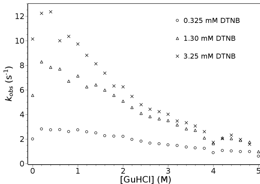
Figure 2. Observed rates of reaction, k_{obs} , of L-cysteine ( 6.5 \mu\text{M} ) with three different concentrations of DTNB (0.325 mM, 1.30 mM, and 3.25 mM) in the presence of increasing concentrations of GuHCl.
