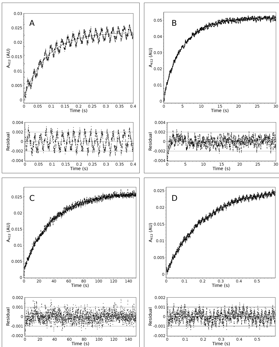
Figure 5. Sample kinetic traces of the four different hRXR \alpha LBD mutants fitted to equation 1. (A) 5.1 \mu M MutC269, 2.54 mM DTNB, no GuHCl. \Delta A_{412} = 0.0224 , k_{obs} = 11.63 \text{ s}^{-1} . (B) 5.2 \mu M MutC369, 1.80 mM DTNB, 1.2 M GuHCl. \Delta A_{412} = 0.0474 , k_{obs} = 0.1945 \text{ s}^{-1} . (C) 4.3 \mu M MutC404, 0.864 mM DTNB, 1.0 M GuHCl. \Delta A_{412} = 0.0233 , k_{obs} = 0.02627 \text{ s}^{-1} . (D) 4.0 \mu M MutC432, 0.802 mM DTNB, 2.2 M GuHCl. \Delta A_{412} = 0.0250 , k_{obs} = 4.83 \text{ s}^{-1} . Residuals shown underneath each trace.
