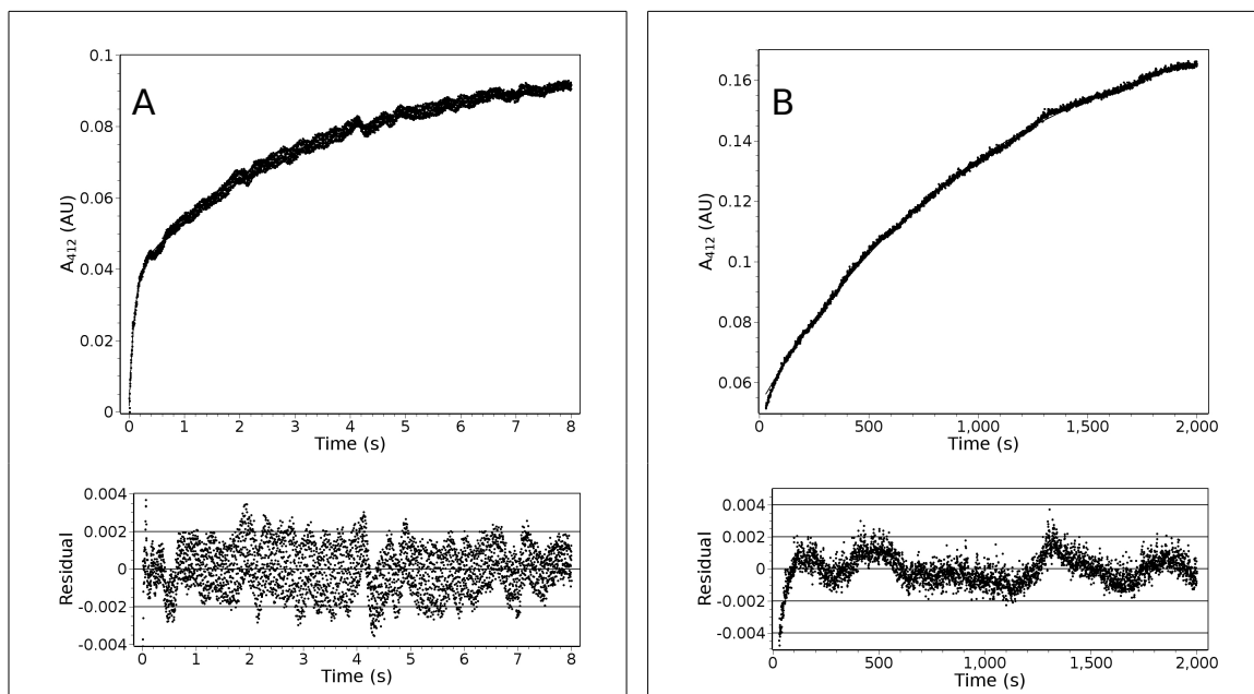
Figure 12. Alkylation of the wild-type hRXR \alpha LBD by DTNB under native conditions. 5.6 \mu M hRXR \alpha LBD and 1.11 mM DTNB. (A) Fast region fitted to eq. 2: D_1 = 0.0365 \pm 0.0004 AU, D_2 = 0.0578 \pm 0.0001 AU, k'_{obs} = 10.7 \pm 0.2 s ^{-1} , k''_{obs} = 0.310 \pm 0.002 s ^{-1} , (B) Slow region fitted to eq. 1: B = 0.1340 \pm 0.0001 AU, k'_{obs} = 0.000934 \pm 0.000002 s ^{-1} .
