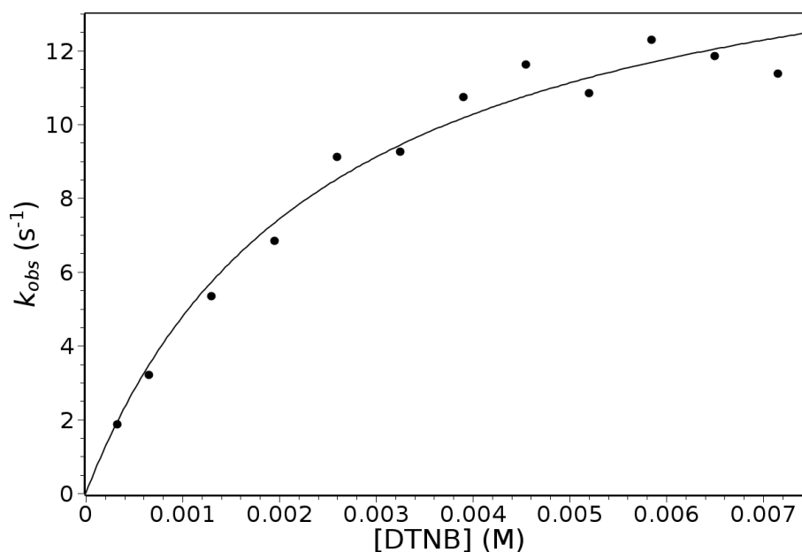
Figure 1. Observed rates of reaction of 6.5 \mu\text{M} L-cysteine with increasing concentrations of DTNB fitted to eq. 4: k_c = 16.6 \pm 1.0 \text{ s}^{-1} and \xi = 2.47 \pm 0.40 \text{ mM} .
