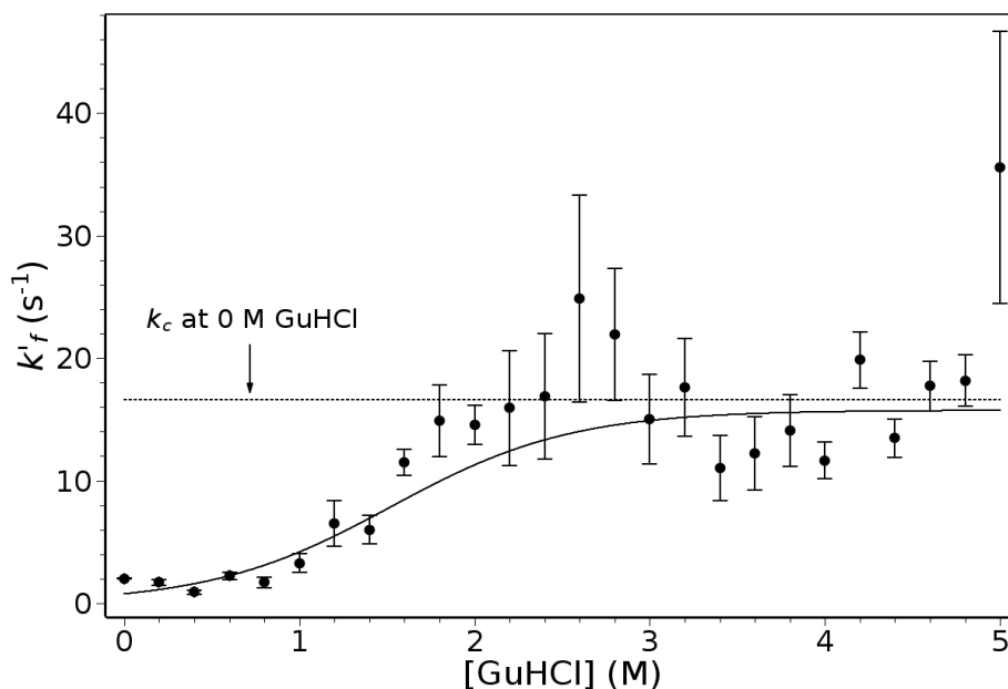
Figure 9. Titration of MutC432 with GuHCl. Maximum rates of reaction, k'_f , were obtained from fitting the corrected (using L-Cys normalization factors) observed rates of reaction, k_{obs} , to eq. 8. Unfolding transition fitted using equations 9 and 11: m = 1,170 \pm 210 cal/mol·M, \Delta G^\circ(\text{H}_2\text{O}) = 1,780 \pm 170 cal/mol, k_f = 15.8 \pm 1.6 s -1 .
