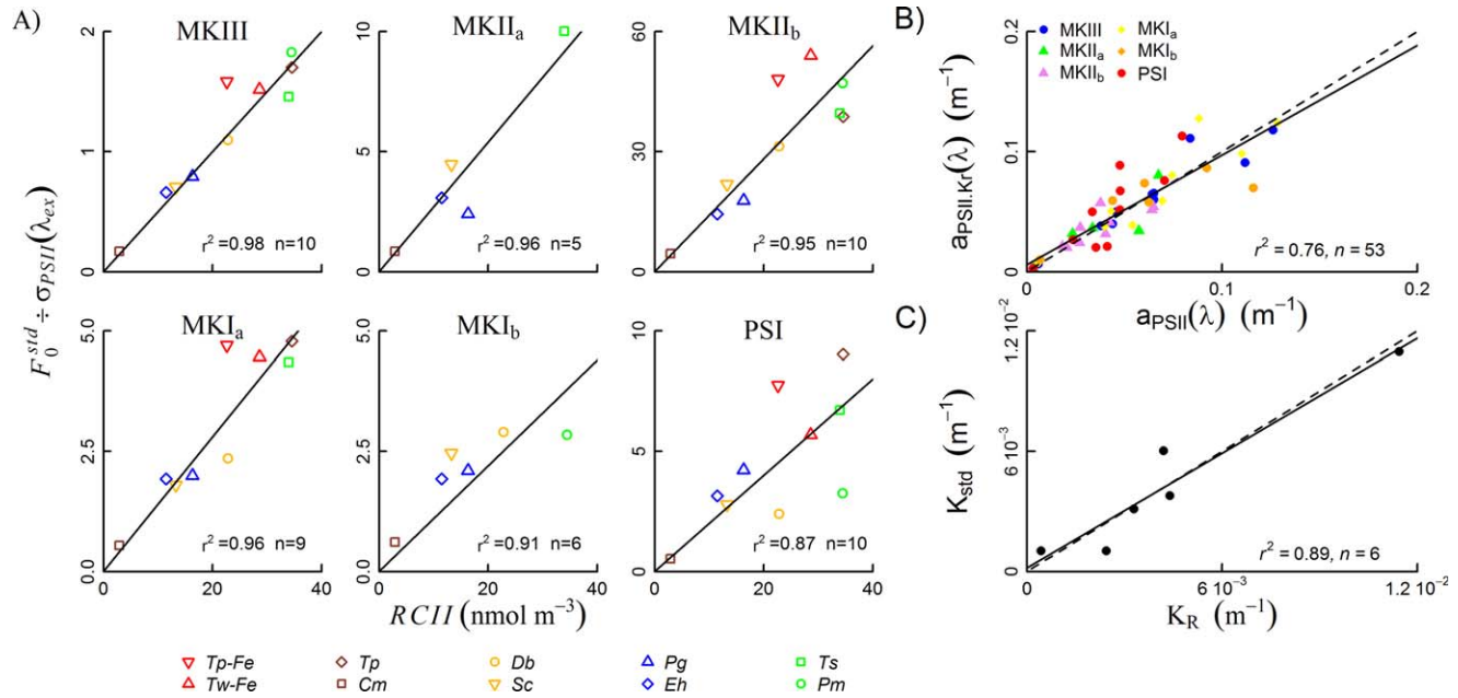
Fig. 6. A: RCII concentrations vs. F_0^{std} / \sigma_{PSII}(\lambda_{ex}) for each culture across six FRRFs. B: Covariance of a_{PSII}(\lambda_{ex}) and a_{PSII,Kr}(\lambda_{ex}) across cultures and instruments. C: Comparison of K_R and K_{std} for the six FRRFs. In (B) and (C) the dashed line represents equivalency and the solid line is the linear regression.
