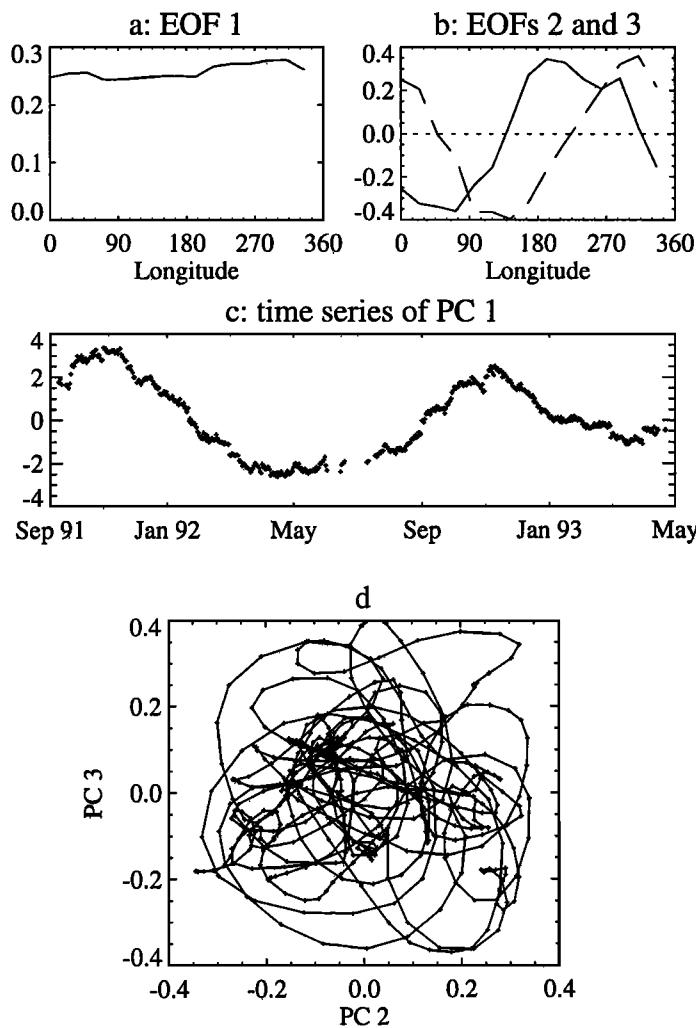
Figure 3. Empirical orthogonal functions of equatorial water vapor at 68 h Pa (a–b) and the time series of their principal components (c–d). In Figure 3b, EOF 2 is indicated by the solid curve, EOF 3 by the dashed curve. In Figure 3d, the (slightly smoothed) principal component time series of EOFs 2 and 3 are plotted against each other to emphasize their phase relationship.
