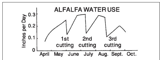
Figure 2.—Typical growing season crop water use by alfalfa.
