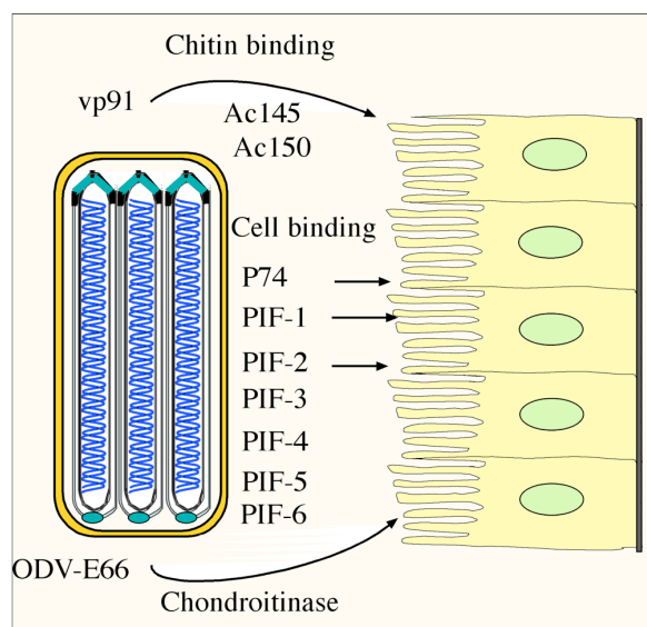
Figure 4. Possible interactions of selected ODV envelope proteins and vp91 (Ac83) with midgut cells. VP91 (Ac83), Ac145 and Ac150 all have chitin binding domains, suggesting that they may interact with chitin synthesizing cells. P74, PIF-1 and -2 bind to midgut cells. The role of PIF-3, 4, 5 and 6 are not known. ODV-E66 has an enzymatic activity (chondroitinase) (27) that may assist in initiating the infection.
