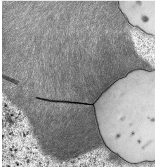
Figure 4. Fibrous p10-containing material aligned with the calyx/polyhedron envelope. Photo courtesy of G. Williams. From (211), with permission.
