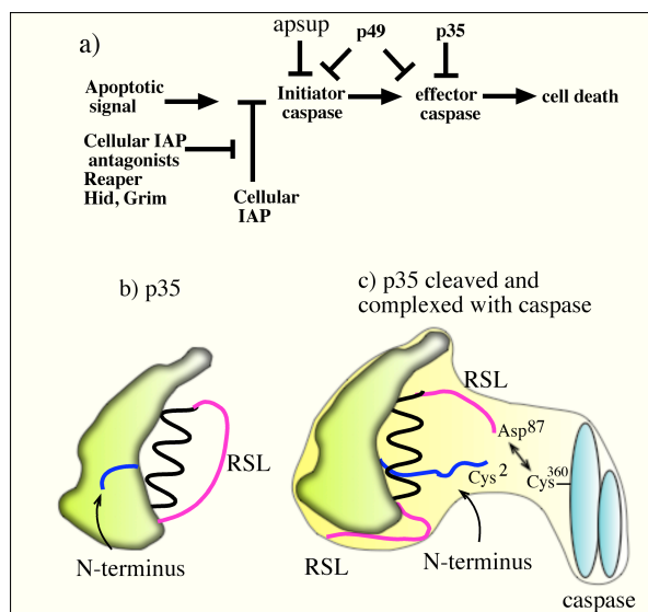
Figure 2. Cell death regulation by p35. a) Baculovirus apoptotic inhibitors P49 and P35 prevent apoptosis by blocking caspase activity. b) Intact P35 showing the reactive site loop and N-terminus which is buried in the P35 structure. c) Cleavage and binding of p35 to caspase-8. P35 cleaved by caspase-8 at Asp 87 . Asp 87 forms a thioester bond with Caspase Cys 360 which is in the proteolytic site, thereby inactivating its enzymatic activity. Cleavage causes the N terminus of P35 to relocate near Asp 87 . Cys 2 near the N-terminus of P35 can also form a thioester with Asp 87 forming a cyclic protein. This diagram is interpreted from (52, 53).
