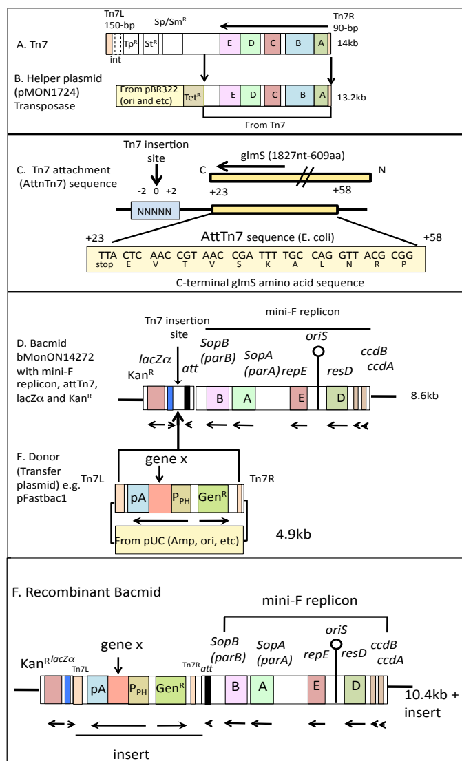
Figure 1. Maps of major constructs used for the production of the bacmid system. A) Map of Tn7. Shown are the genes A-E that are involved in transposition (see text) and at the left end int associated with an inactive integron system and three antibiotic resistance genes including Tp r (trimethoprim), streptothricin St r , and streptomycin and spectinomycin Sp/Sm r (36) (35). B.) Map of the helper plasmid showing the components of Tn7 used in its construction. C) Tn7 attachment sequence. Map of the C-terminal end of the glmS gene showing the Tn7 insertion site 21-25 nt downstream. D). This map shows the organization of the integration site along with the region from the fertility (F) plasmid (mini F-replicon). The genes shown are involved in the coordination of the replication of the bacmid with the bacterial genome (see text). Also shown is the Tn7 integration site ( att ) and the kanamycin resistance gene ( Kan r ) and lacZα . E.). Map of the donor (transfer) plasmids such as pFastbac1. The location of the polyadenylation signal ( pA ) polyhedrin promoter ( P PH ), the selectable marker gentamicin resistance ( Gen r ) along with the location of the gene being expressed (gene x ). The sequences involved in integration into the att site, Tn7L and Tn7R, are also shown. The rest of the map are the components of the pUC plasmid used for making the transfer plasmid). F.). This is a map of an example of a recombinant bacmid. For abbreviations see above.
