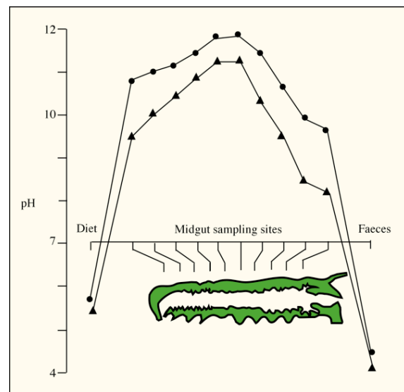
Figure 3. PH profiles along the gut lumens of two lepidopteran species. The pH of the hemolymph was 6.7. The species shown are Lichnoptera felina (circles) and Manduca sexta (triangles). This figure is reproduced with permission of the Company of Biologists from (3).
