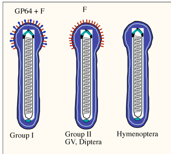
Figure 6. Distribution of envelope fusion proteins. Group I have homologs of both GP64 and F, but F is not a fusion protein. Group II, GVs and dipteran viruses have homologs of F, whereas the hymenopteran viruses have homologs of neither GP64 nor F.
