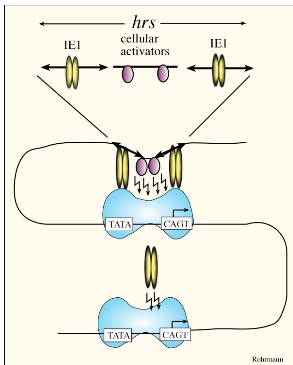
Figure 3. Activation of baculovirus early gene transcription by hrs and IE1. This diagram shows two possible mechanism by which IE1 activates transcription. Transcription might be activated directly by IE1 as shown in the bottom of the diagram, or it can interact with both RNA polymerase II (in blue) and hrs sequences thereby bringing hrs -bound transcriptional activators in close proximity to RNA polymerase II as shown in the top of the figure.
