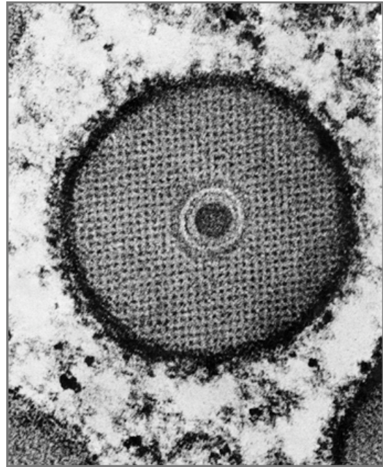
Figure 4. Cross section of a granulovirus of Plodia interpunctella . From Arnott and Smith (80). Copyright Elsevier 1967. Reproduced with permission via Copyright Clearance Center.
