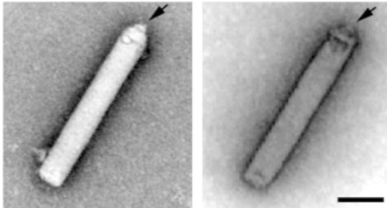
Figure 9. Morphology of AcMNPV capsids stained with uranyl acetate. The figure shows the morphology of the two ends, one with a conical shape (arrow). Scale bar, 50 nm .From Au and Pante (213). Reproduced with permission of Elsevier Limited via Copyright Clearance Center.
