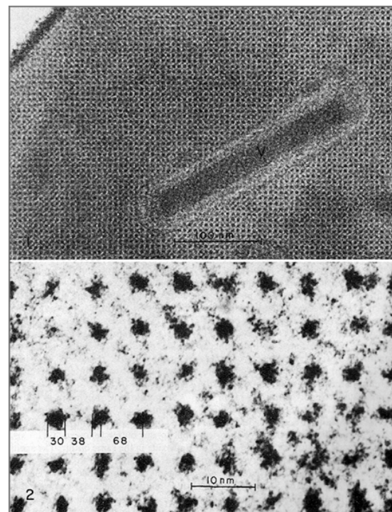
Figure 1. Sections of portions of polyhedra showing crystalline structure. Top panel is from an NPV of Pseudohazis eglanterina (pine butterfly). Bottom panel is a higher magnification from an NPV of Nemytia freemani (false hemlock looper). Measurements are shown in Angstroms. From K. Hughes (210). Reproduced with permission of Elsevier Limited via Copyright Clearance Center.
