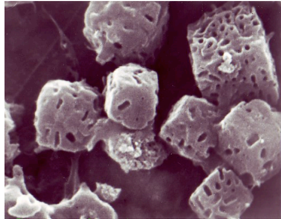
Figure 5. Polyhedra from OpMNPV with the polyhedron envelope protein and p10 genes deleted. From (13), with permission.
