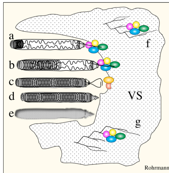
Figure 2. Theoretical diagram of different stages of DNA replication and packaging. Shown is replication coordinated with packaging (a and b) and DNA replication that is independent of packaging showing extensive recombination (f,g). The large stippled area is the virogenic stroma (VS). The circularization of the genome by recombination is also indicated (c). Mature virions are represented by (d) and (e).
