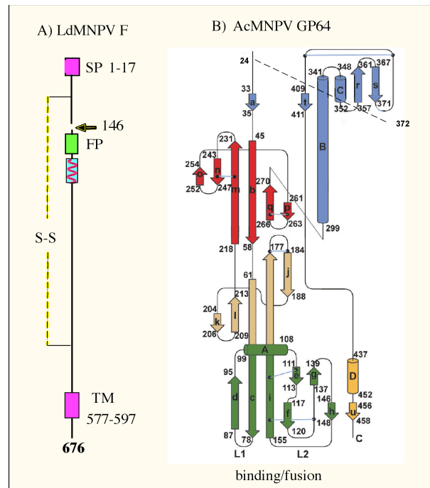
Figure 7. Structure of the baculovirus F (fusion) protein (Ld130) from LdMNPV and AcMNPV GP64. A) Ld130 F protein. Shown is a predicted signal peptide (SP), fusion peptide (FP) and transmembrane domain (TM) including the amino acid coordinates. The cleavage site is indicated by the arrow. A predicted coiled coil domain is also indicated. The disulfide bond is predicted from (212). B) GP64. This figure is derived from Kadlec (60). Shown are 7 disulfide bonds, all of which are intramolecular except for the one from aa 24 which is connected to aa 372 in an adjacent molecule. This and the coiled-coil (299-341) region are involved in trimer formation. All the disulfide bonds are conserved except 178-184 which is not present in thogotovirus GP64. The receptor binding/fusion peptide region is shown at the base of the diagram. From Kadlec et al (60). Copyright 2008 by Nature Publishing Group. Reproduced with permission of Nature Publishing Group via Copyright Clearance Center.
