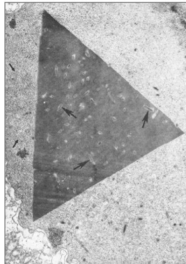
Figure 6. Polyhedral inclusion body of a virus of the pink shrimp, Penaeus monodon . Arrows indicated nucleocapsids. From Couch (16). Reproduced with permission of Elsevier Limited via Copyright Clearance Center.
