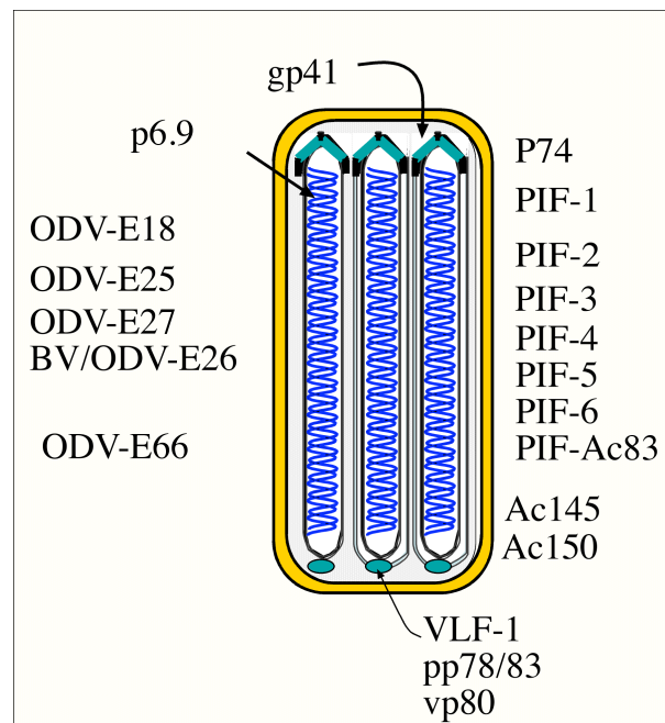
Figure 8. Selected structural proteins of ODV. Shown are envelope associated proteins (ODV-E), the PIF proteins (also envelope associated), the tegument protein, gp41, the DNA binding protein, p6.9, and two basal end-associated proteins, pp78/83 and VLF-1. For convenience, VLF-1 and Vp80 is shown here located at the basal end, however, they could be located at the apical end (199) (146). There are a variety of other capsid proteins, but they appear to have a more generalized distribution. For details see the text.
