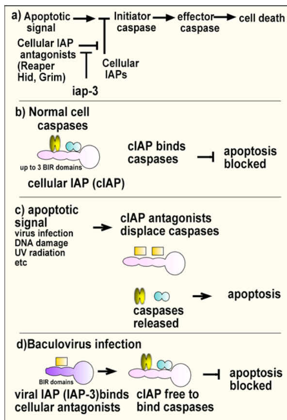
Figure 3. A possible mechanism for baculovirus IAP to block apoptosis. a) Schematic diagram of theory. b) Cellular IAP (cIAP) is related to baculovirus IAP and in the normal cells blocks apoptosis by sequestering caspases. c) Upon induction of apoptosis, cIAP antagonists displace caspases. This frees up the caspases to cause apoptosis. d) It is thought that baculovirus IAP blocks apoptosis by binding cIAP antagonists, thereby freeing up cIAP to bind caspases.
