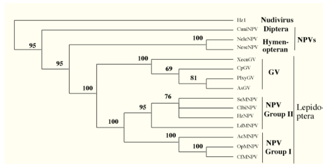
Figure 5. Phylogenetic relatedness of LEF8 from selected baculoviruses.
