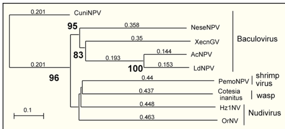
Figure 7. Phylogenetic relatedness of VLF-1 from selected viruses and a braconid wasp. Neighbor joining Best Tree; Numbers in bold indicate Bootstrap values (1000 reps) over 50%. Abbreviations: PemoNPV, Penaeus monodon (shrimp); Cotesia inanitus (braconid wasp); Hz1NV and OrNV, nudiviruses.
