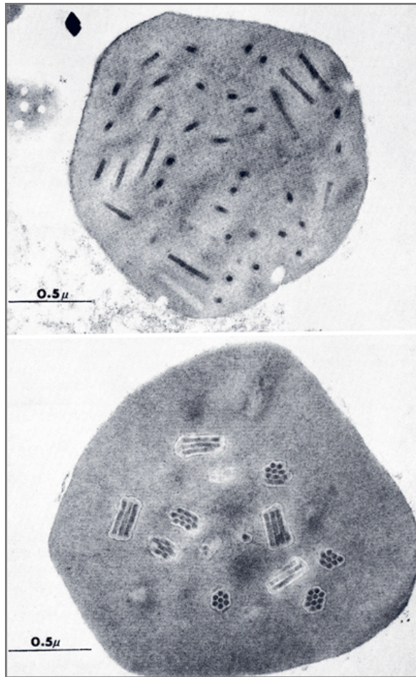
Figure 3. Two nucleopolyhedroviruses pathogenic for Orgyia pseudotsugata showing single (top panel) and multiple (bottom panel) nucleocapsids/envelope. From Hughes and Addison (37). Copyright 1970 Elsevier. Reproduced with permission via Copyright Clearance Center.
