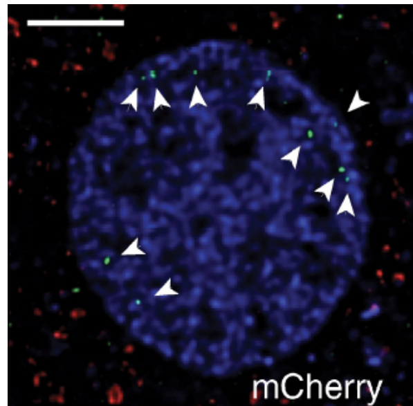
Figure 6. Entry of AcMNPV nucleocapsids through nuclear pores. This shows virus with the capsid protein VP39 fused with the fluorescent label, mCherry. Arrows indicate capsids; bar is 5 mm. ©Ohkawa et al., 2010. Originally published in J. Cell Biol. 190:187-195.
