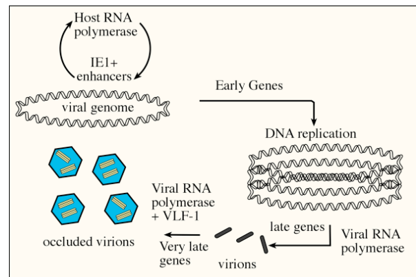
Figure 1. The baculovirus transcriptional cascade showing the interrelationship of host and viral RNA polymerases and DNA replication and VLF-1.
