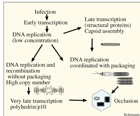
Figure 3. Hypothetical diagram for roles of two types of baculovirus DNA: genomic DNA that is packaged and DNA that is not packaged and is essential for very late transcription.
