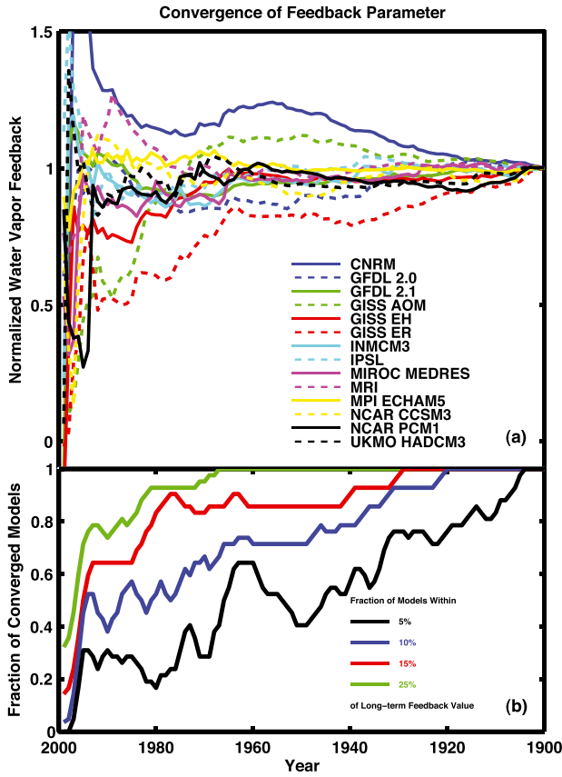
Figure 5. (a) Normalized water vapor feedback values for the 14 AOGCMs calculated using different record lengths, starting from the end of the record in year 2000 and proceeding back in time. Each value is normalized by the corresponding water vapor feedback for the entire twentieth century. (b) Fraction of models that attain a short-term feedback value within 5% (black), 10% (blue), 15% (red), and 25% (green) of the long-term value for each model. A 3 year box smoothing is applied to make the figure more readable.
