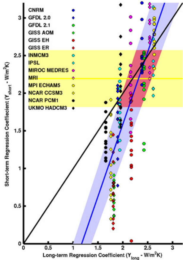
Figure 6. Comparison between the calculations of short-term water vapor feedback ( Y_{short} ) for distinct 88-month periods with the long-term water vapor feedback ( Y_{long} ) for 14 different AOGCMs. The blue line represents an ordinary least squares fit for all models, with the blue shaded region representing the 95% confidence interval for this regression. The solid black line is a one-to-one line for reference. The yellow shaded region represents the estimate in Y_q from the AIRS observations, with 95% confidence intervals. The red region represents an estimate of the range of possible values for the long-term water vapor feedback.
