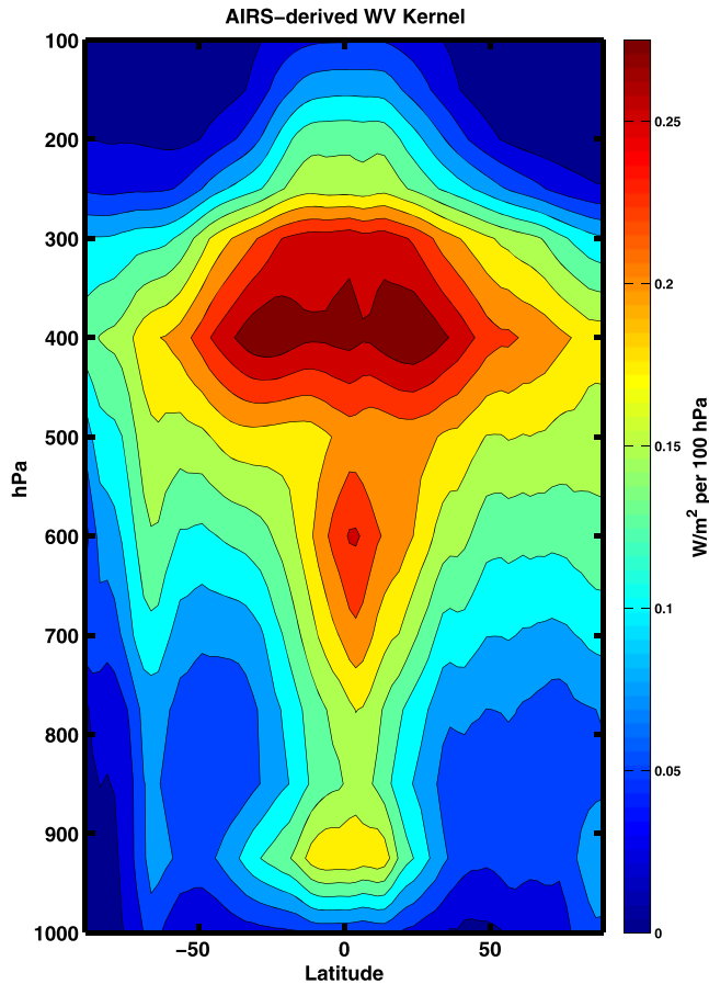
Figure 3. Zonal average of change in net TOA irradiance for a unit perturbation in water vapor that corresponds to a 1 K temperature change with fixed relative humidity ( \text{Wm}^{-2} per 100 mb).
