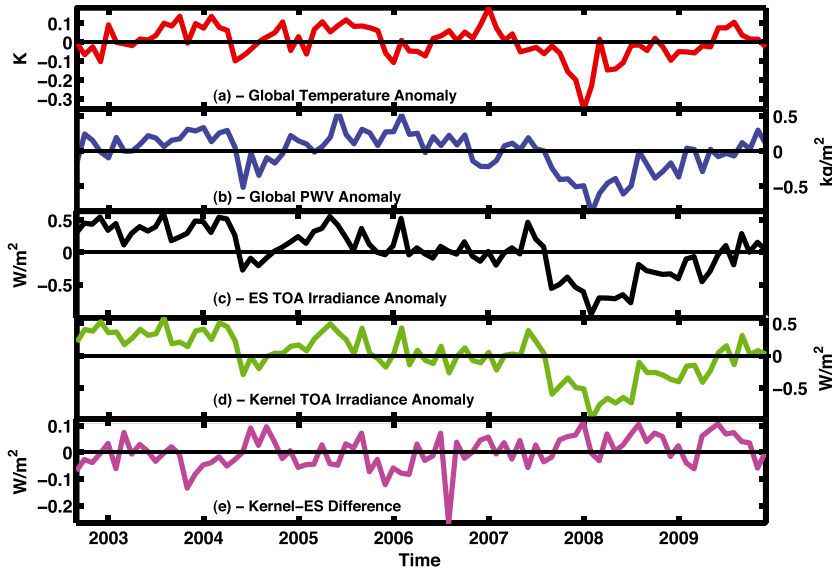
Figure 1. Time series for the AIRS observational period (September 2002–December 2009) of (a) global mean surface temperature anomaly (with respect to mean of time period) from HadCRUT3 data set, (b) AIRS-derived global mean precipitable water vapor anomaly, and global mean TOA net irradiance anomaly derived from (c) full integration of the radiation code, (d) kernel calculation, and (e) difference (kernel-ES).
