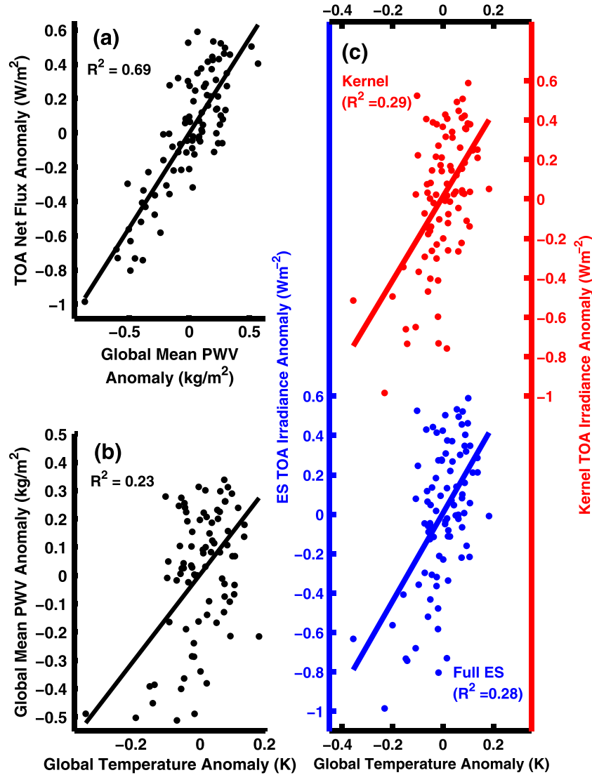
Figure 2. Regressions of (a) satellite-derived global mean precipitable water vapor anomaly and simulated TOA net irradiance anomaly from the radiation code, (b) global mean surface temperature and global mean precipitable water vapor, and (c) global mean surface temperature from HadCRUT3 and TOA net irradiance anomaly for the full radiation code (blue) and for the kernel technique (red).
