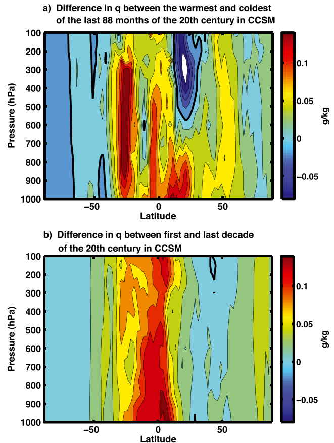
Figure 4. Zonally averaged vertical distribution in moisture anomaly for the Community Climate System Model (CCSM) (a) between the warmest and coldest decade of months in the last 88 months of the twentieth century integration of the CCSM, and (b) between the first and last decade of the twentieth century integration.
